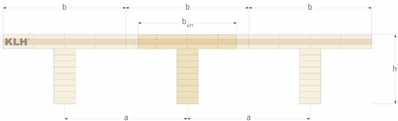
Fig. 5: Dimensions of the T-beam cross-section
