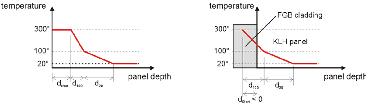
Figure 21: Temperature profiles for non cladded and cladded KLH® - CLT
